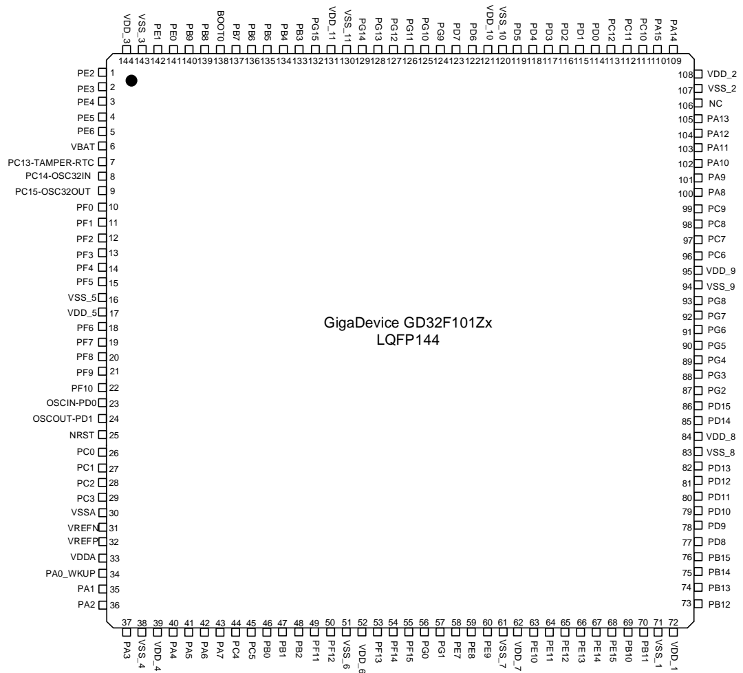
Figure 2-3. GD32F101Zx LQFP144 pinouts
